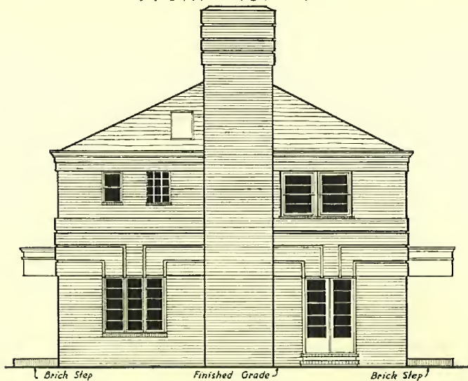
Rear Elevation
